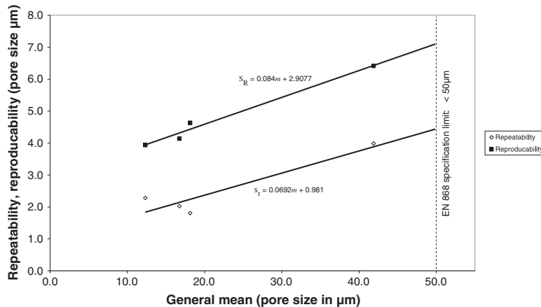
Figure 1. Pore size: plot of repeatability and reproducibility against general mean.
