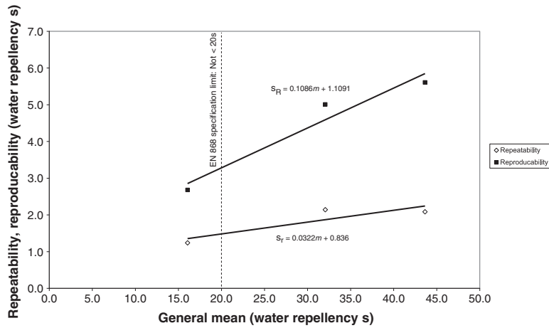
Figure 2. Water repellency: plot of repeatability and reproducibility against general mean.
