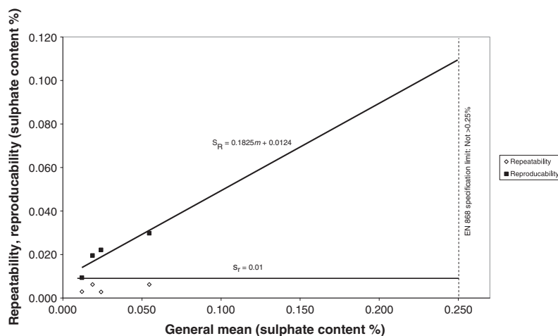
Figure 4. Sulfate content: plot of repeatability and reproducibility against general mean.
