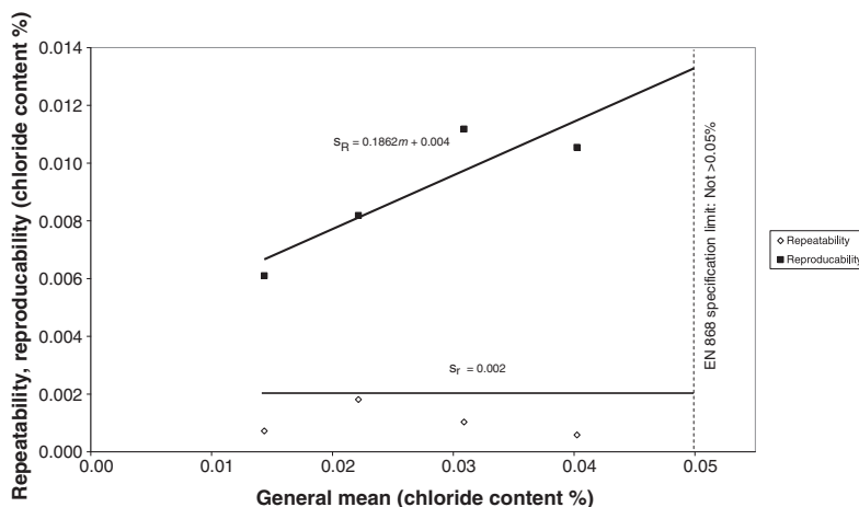
Figure 3. Chloride content: plot of repeatability and reproducibility against general mean.
